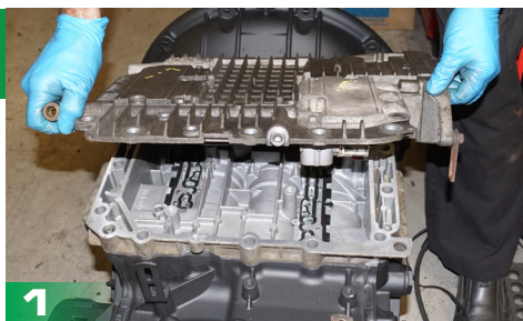
Broken AMT Cylinder Housing Ribbon
